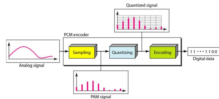
Figure 4.21 Components of PCM encoder
