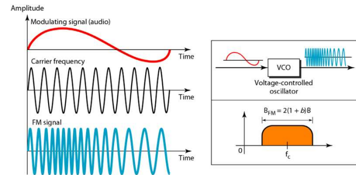
Figure 5.18 Frequency modulation
