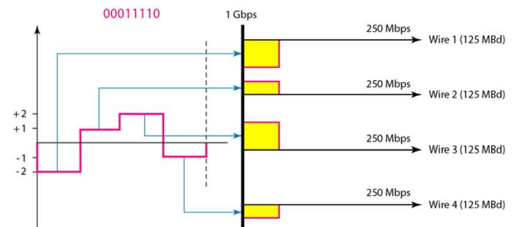
Figure 4.12 Multilevel: 4D-PAM5 scheme
