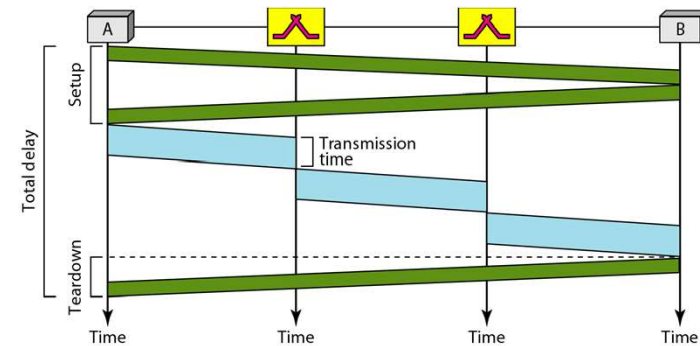
Figure 8.16 Delay in a virtual-circuit network
