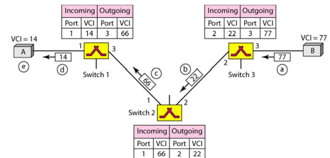
Figure 8.15 Setup acknowledgment in a virtual-circuit network
