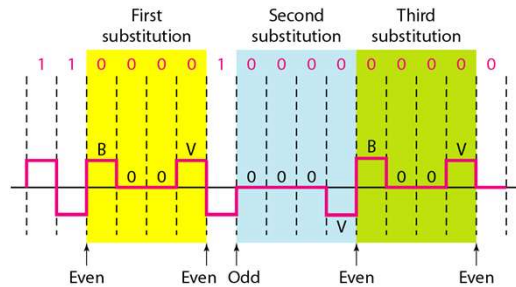
Figure 4.20 Different situations in HDB3 scrambling technique
