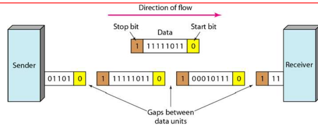
Figure 4.34 Asynchronous transmission
