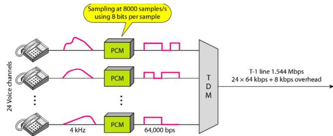
Figure 6.24 T-1 line for multiplexing telephone lines
