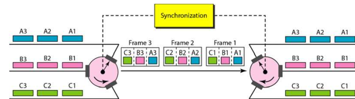
Figure 6.15 Interleaving
