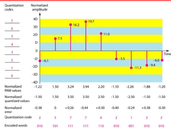
Figure 4.26 Quantization and encoding of a sampled signal
