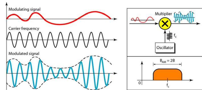
Figure 5.16 Amplitude modulation
