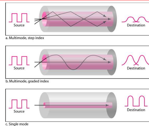
Figure 7.13 Modes
