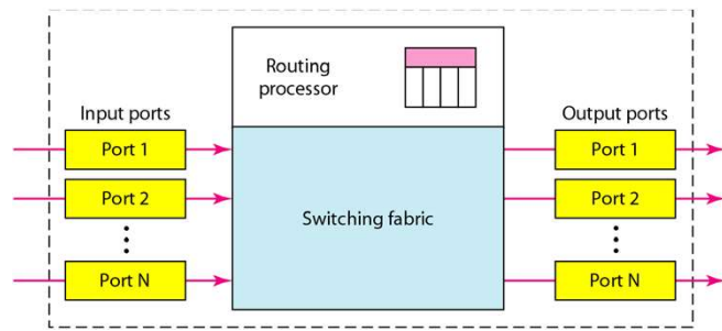
Figure 8.21 Packet switch components
