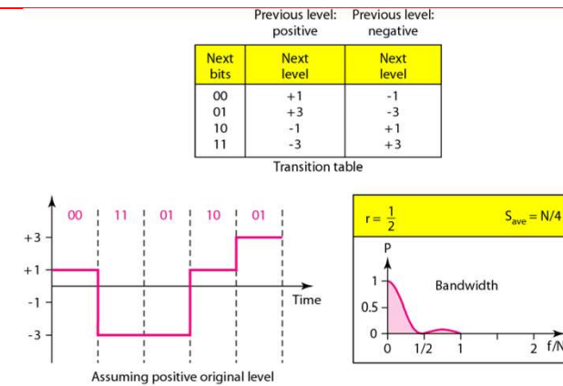
Figure 4.10 Multilevel: 2B1Q scheme
