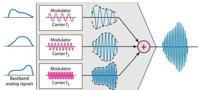
Figure 6.4 FDM process
