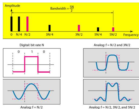
Figure 3.22 Simulating a digital signal with first three harmonics
