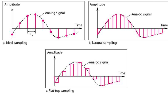
Figure 4.22 Three different sampling methods for PCM
