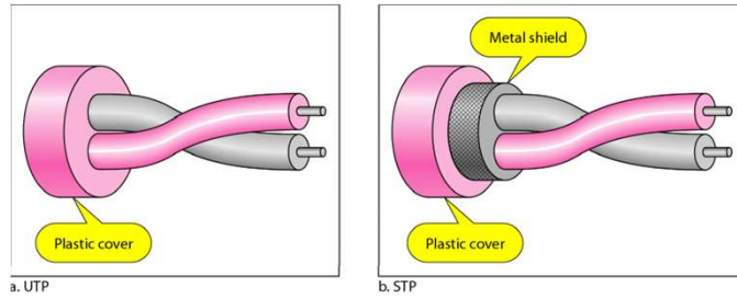
Figure 7.4 UTP and STP cables
