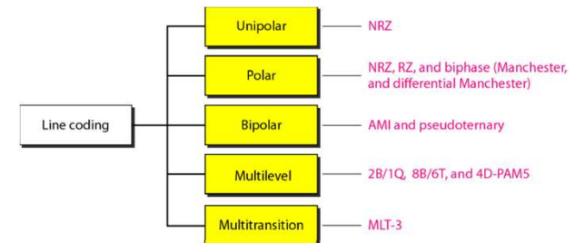
Figure 4.4 Line coding schemes
