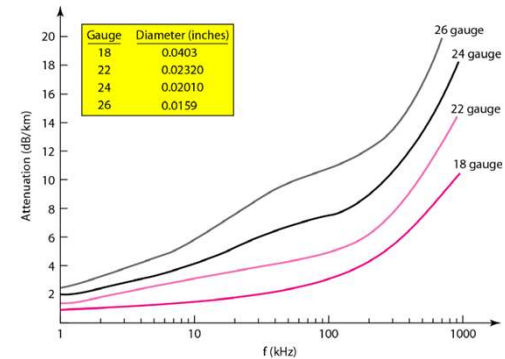
Figure 7.6 UTP performance
