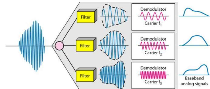
Figure 6.5 FDM demultiplexing example
