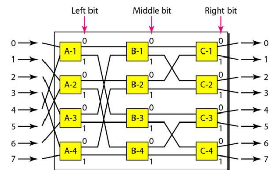
Figure 8.24 A banyan switch
