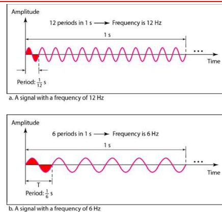
Figure 3.4 Two signals with the same amplitude and phase, but different frequencies
