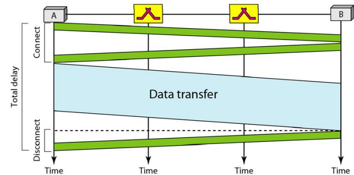
Figure 8.6 Delay in a circuit-switched network
