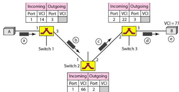
Figure 8.14 Setup request in a virtual-circuit network
