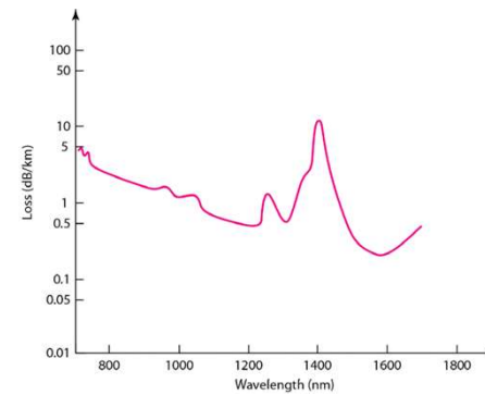
Figure 7.16 Optical fiber performance
