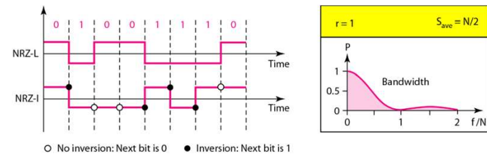
Figure 4.6 Polar NRZ-L and NRZ-I schemes
