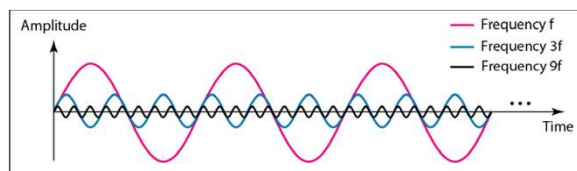
a. Time-domain decomposition of a composite signal
