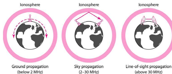
Figure 7.18 Propagation methods
