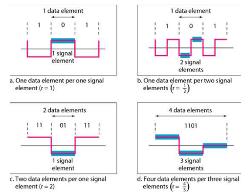
Figure 4.2 Signal element versus data element
