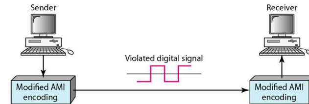
Figure 4.18 AMI used with scrambling
