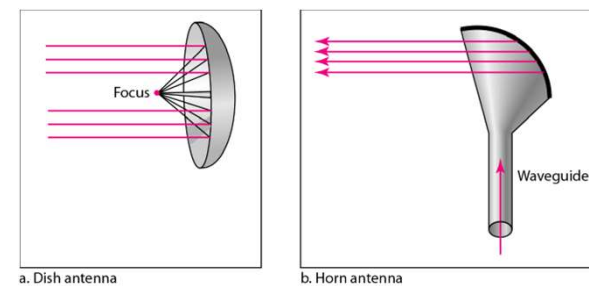
Figure 7.21 Unidirectional antennas
