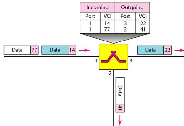
Figure 8.12 Switch and tables in a virtual-circuit network
