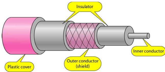
Figure 7.7 Coaxial cable
