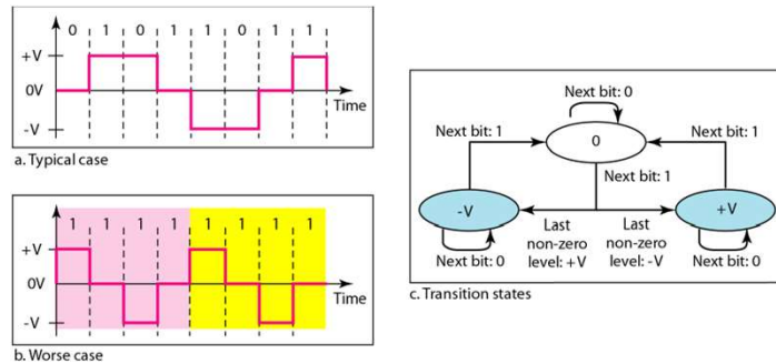
Figure 4.13 Multitransition: MLT-3 scheme
