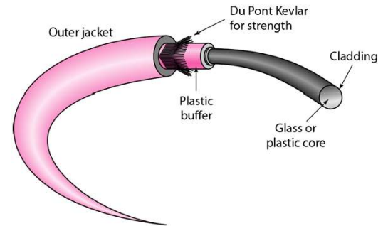
Figure 7.14 Fiber construction
