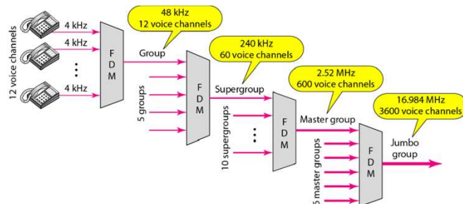
Figure 6.9 Analog hierarchy
