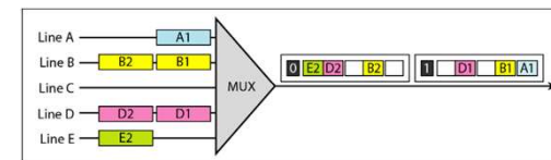
Figure 6.26 TDM slot comparison
