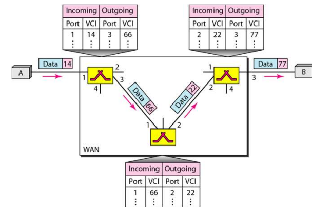
Figure 8.13 Source-to-destination data transfer in a virtual-circuit network
