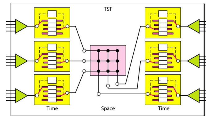
Figure 8.20 Time-space-time switch
