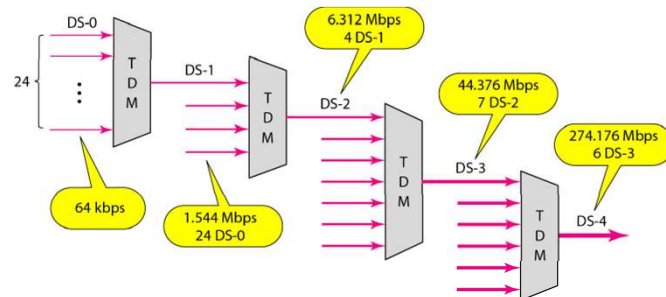
Figure 6.23 Digital hierarchy
