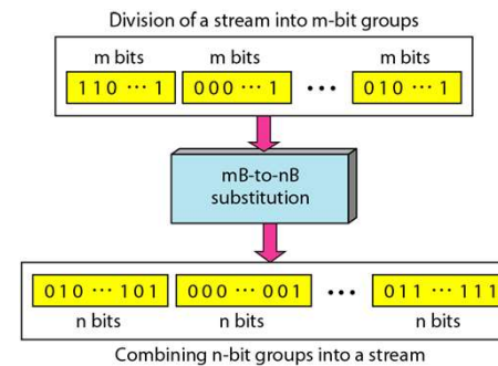
Figure 4.14 Block coding concept
