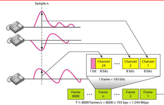
Figure 6.25 T-1 frame structure
