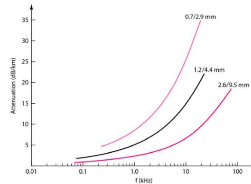
Figure 7.9 Coaxial cable performance
