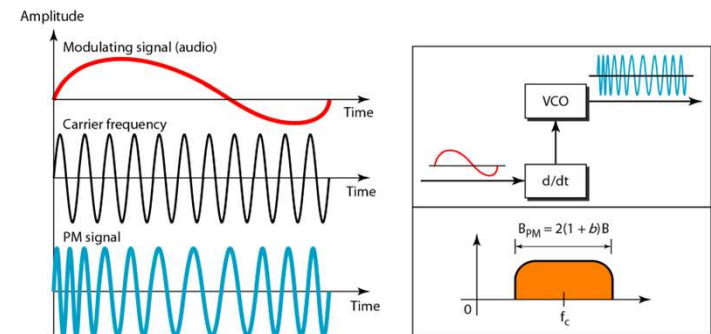
Figure 5.20 Phase modulation
