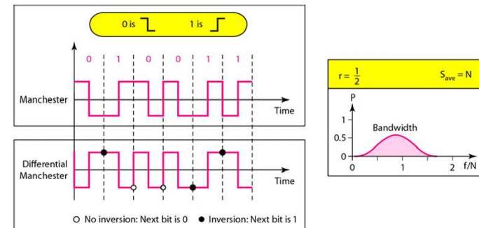
Figure 4.8 Polar biphase: Manchester and differential Manchester schemes
