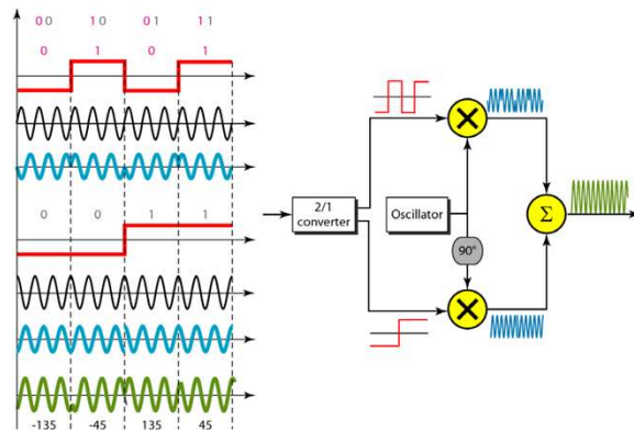
Figure 5.11 QPSK and its implementation
