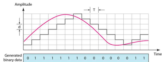
Figure 4.28 The process of delta modulation
