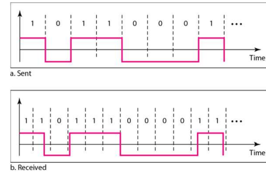
Figure 4.3 Effect of lack of synchronization
